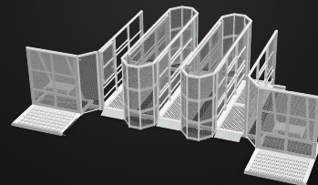
THREE LANES IN A ROW, 3D VIEW
